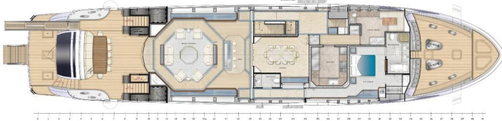
MAIN DECK
