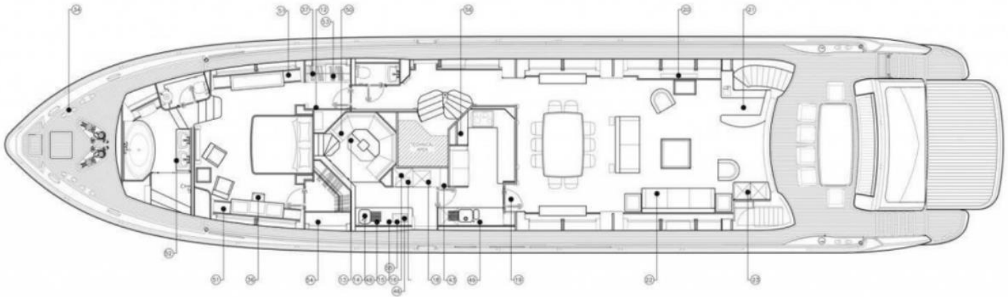
Lower deck
